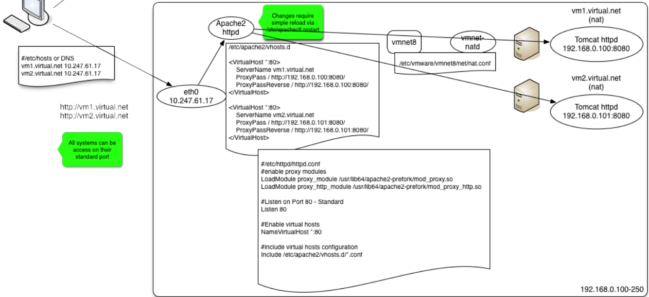
Option 2 : using Apache Reverse Proxy
